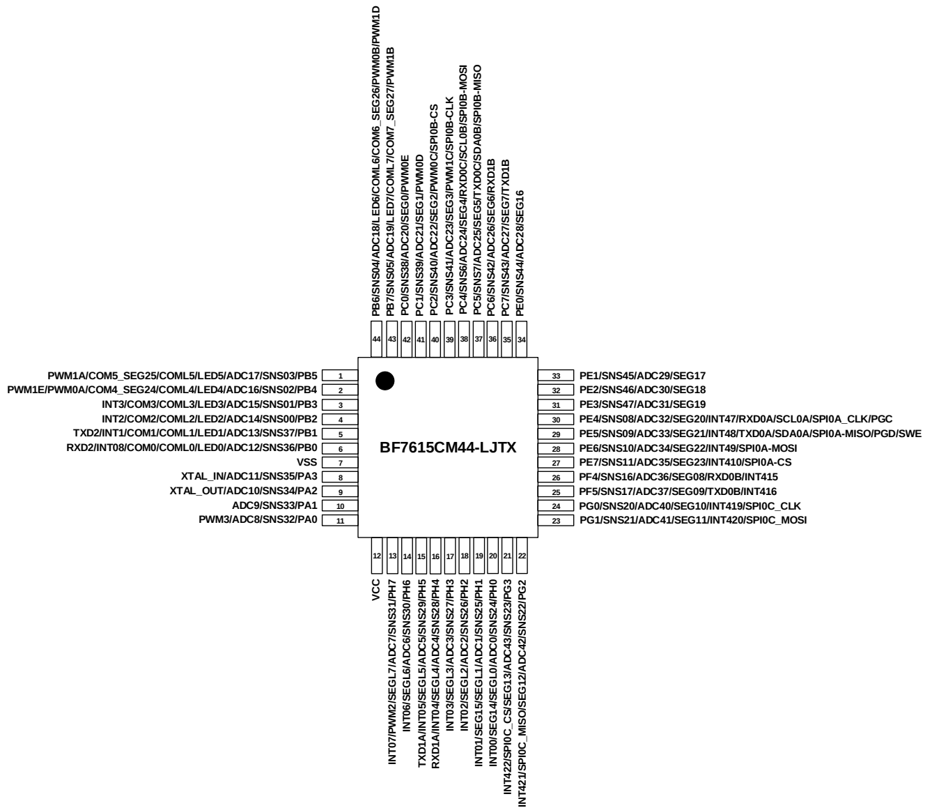
BF7615CM44-LJTX package pin diagram
