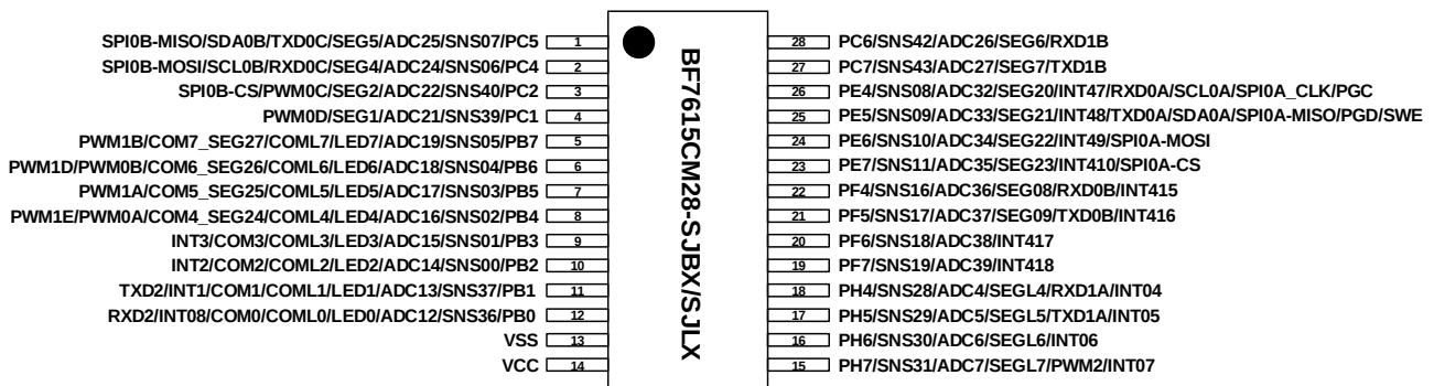
BF7615CM28-SJBX/SJLX package pin diagram
