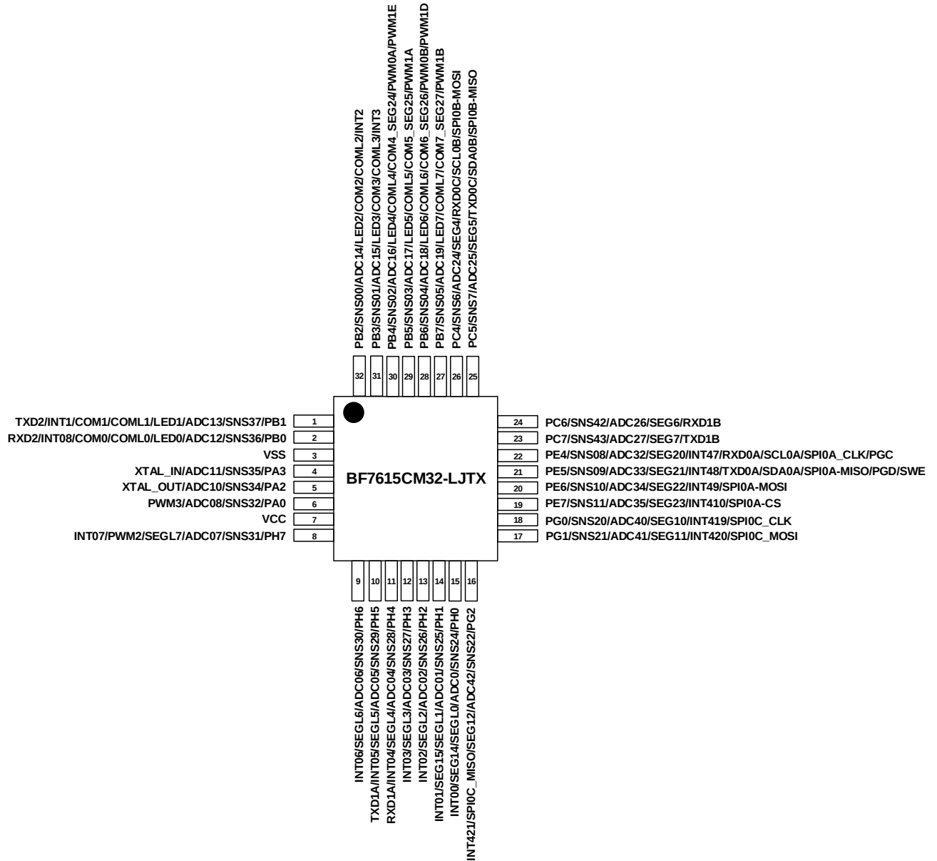
BF7615CM32-LJTX package pin diagram
