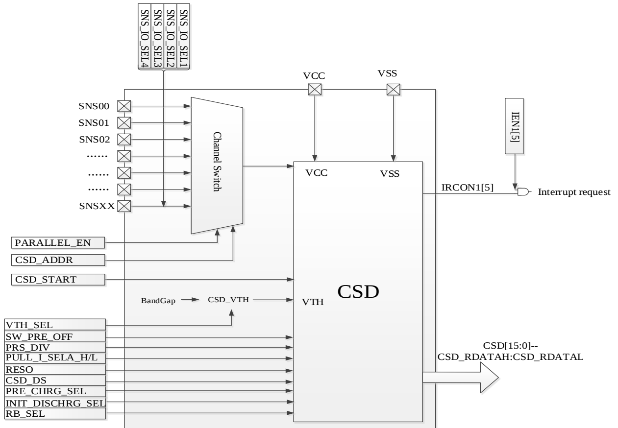
CSD structure diagram
