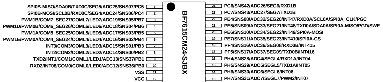
BF7615CM24-SJBX package pin diagram
