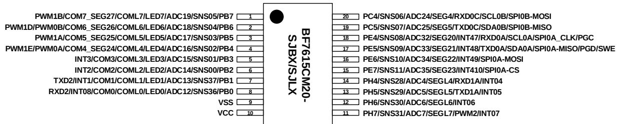
BF7615CM20-SJBX/SJLX package pin diagram
