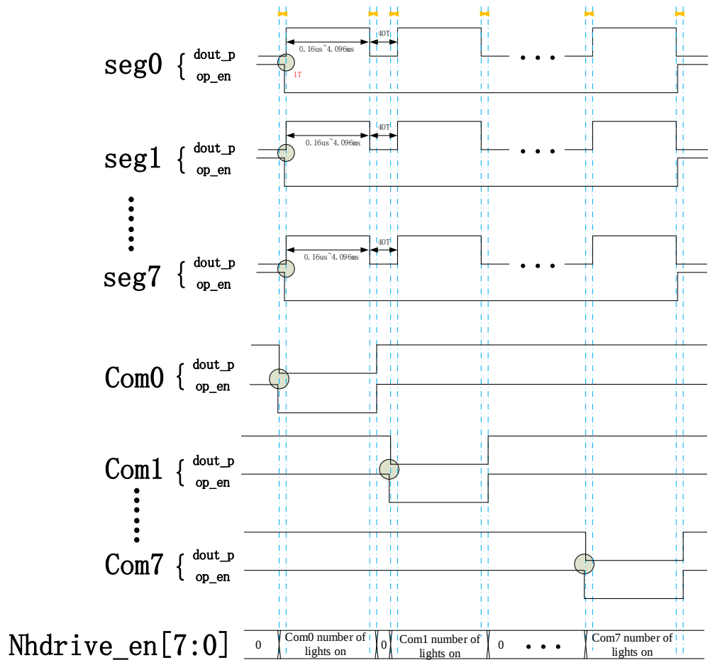
Timing diagram of LED matrix mode
